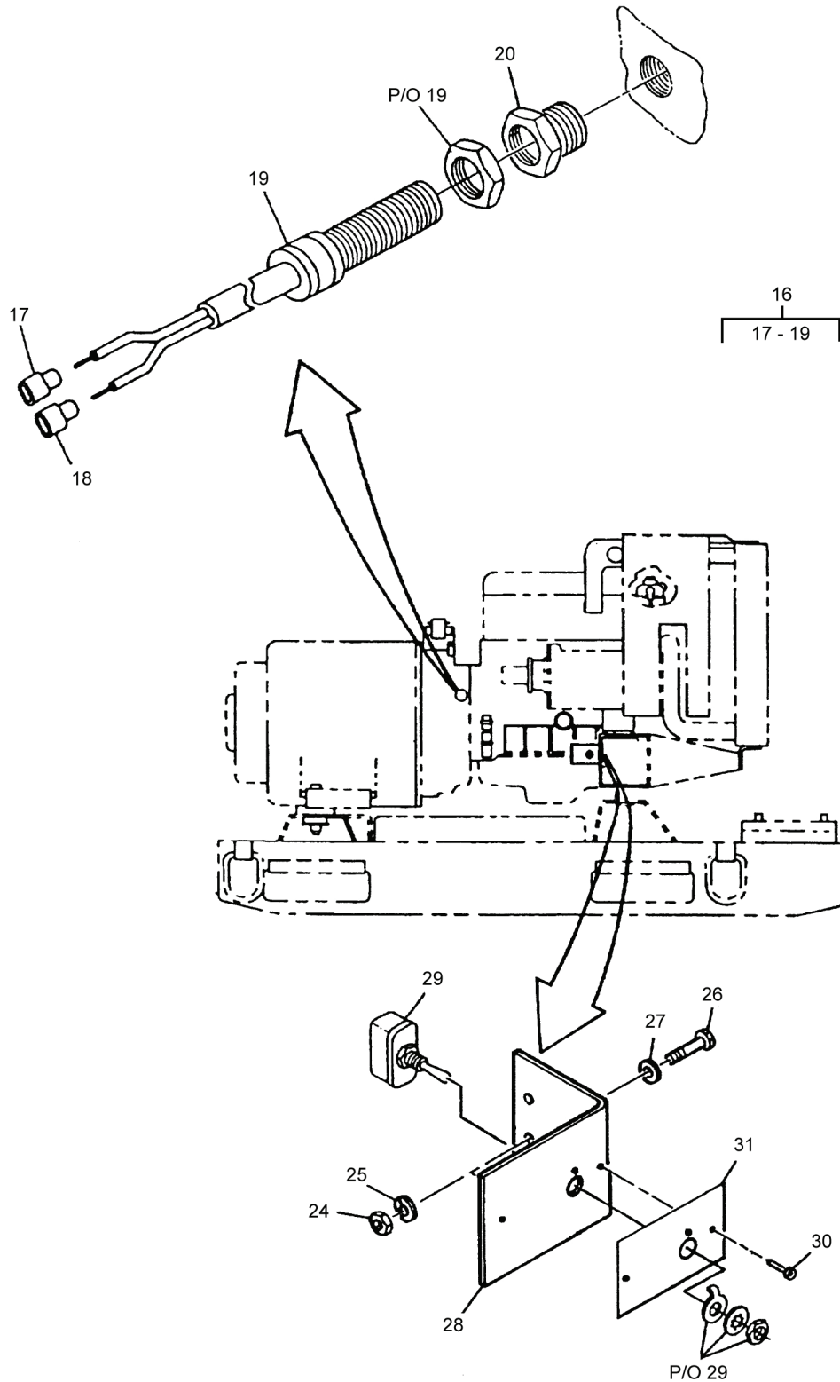
Figure 18. Engine Accessories (Sheet 2 of 5).
