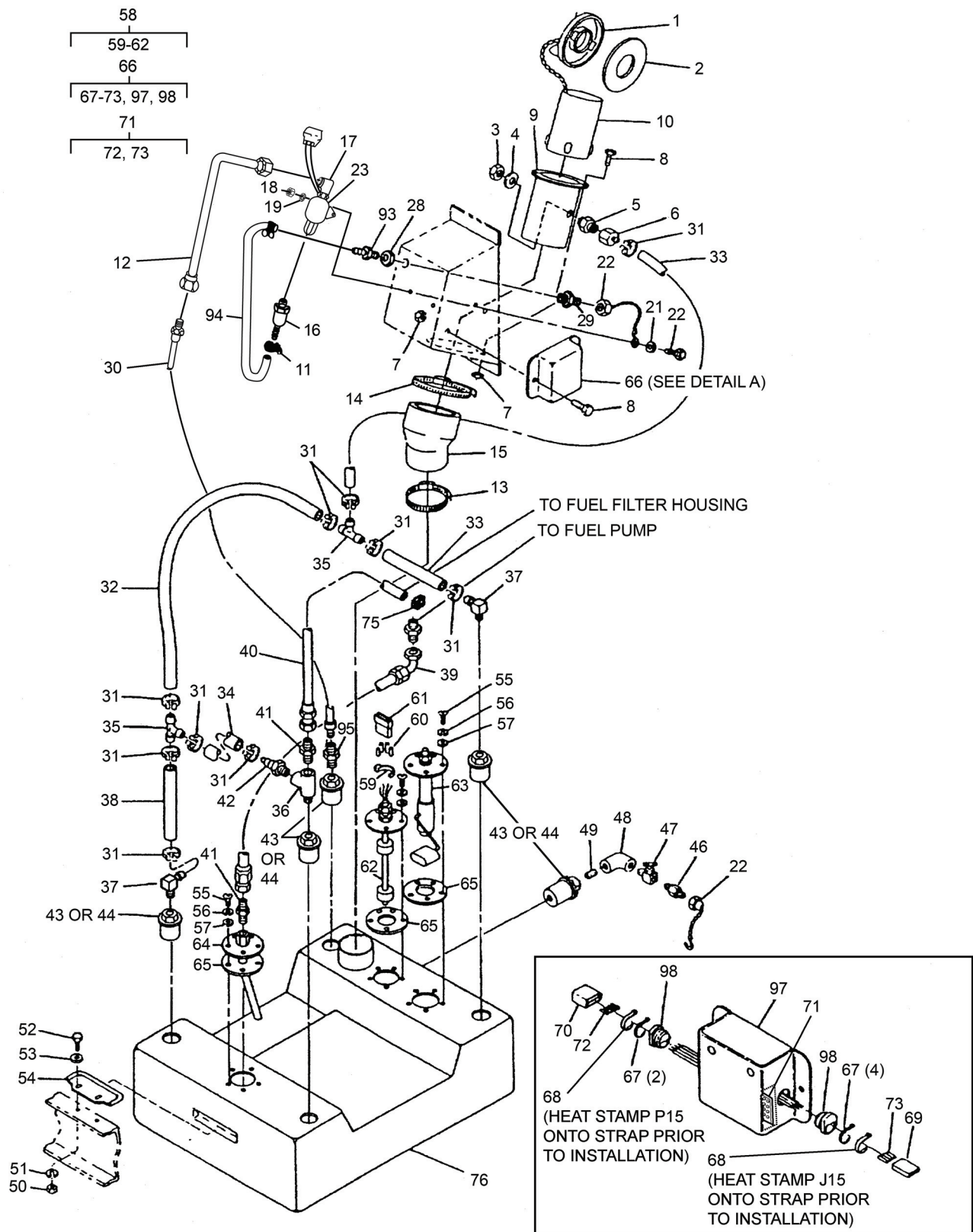
Figure 13. Fuel Tank, Lines and Fittings (Sheet 1 of 2).
