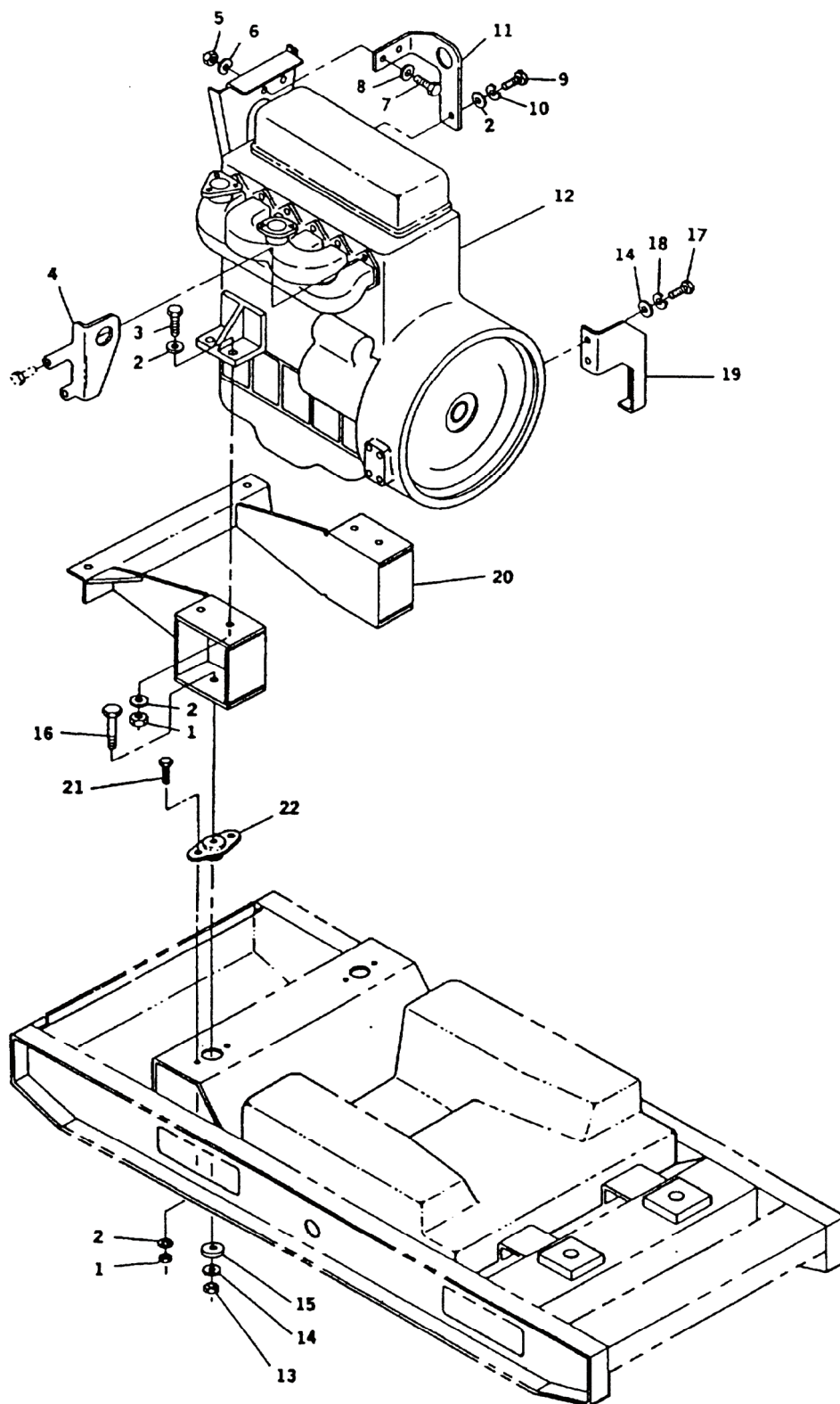
Figure 23. Engine Installation.
