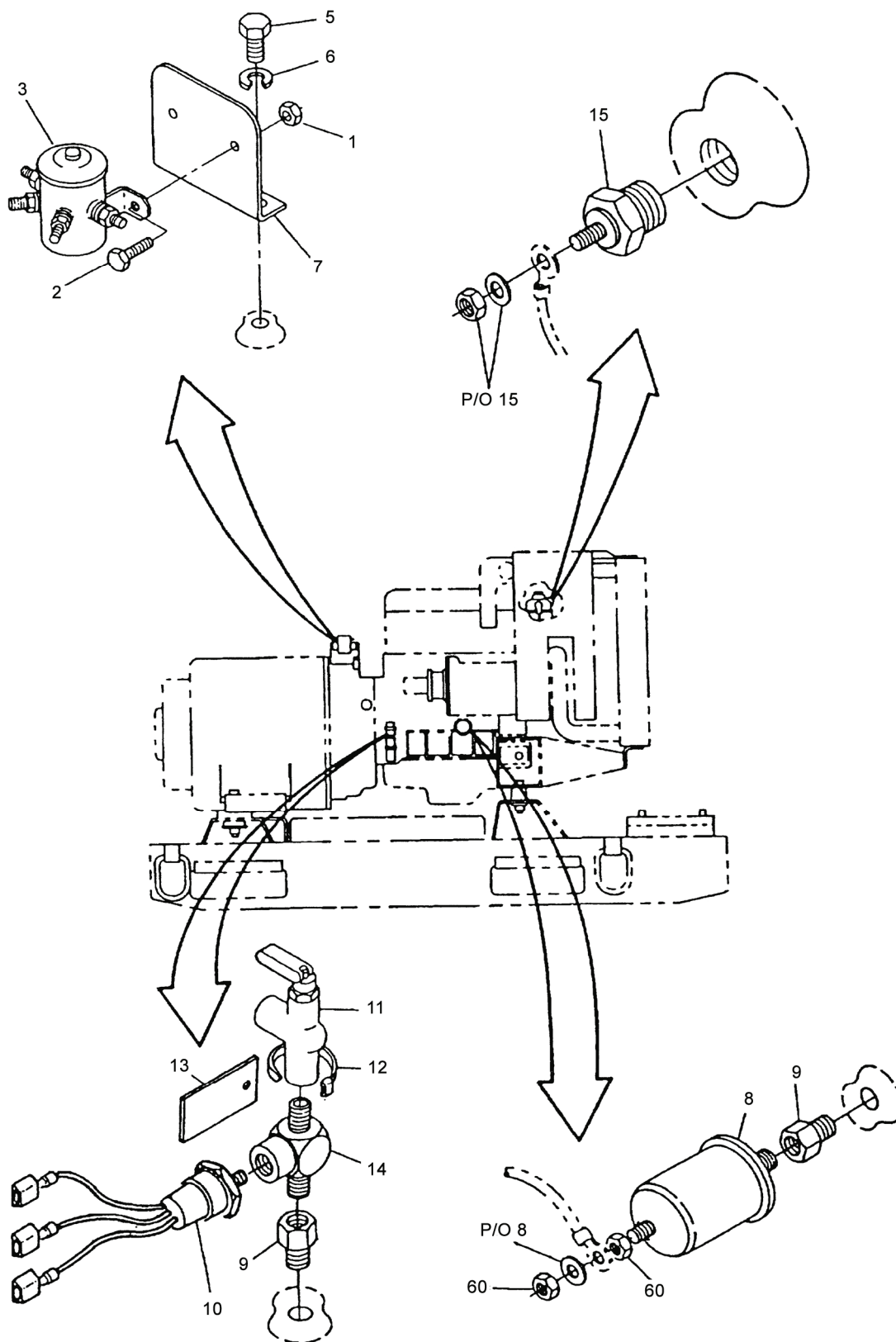
Figure 18. Engine Accessories (Sheet 1 of 5).
