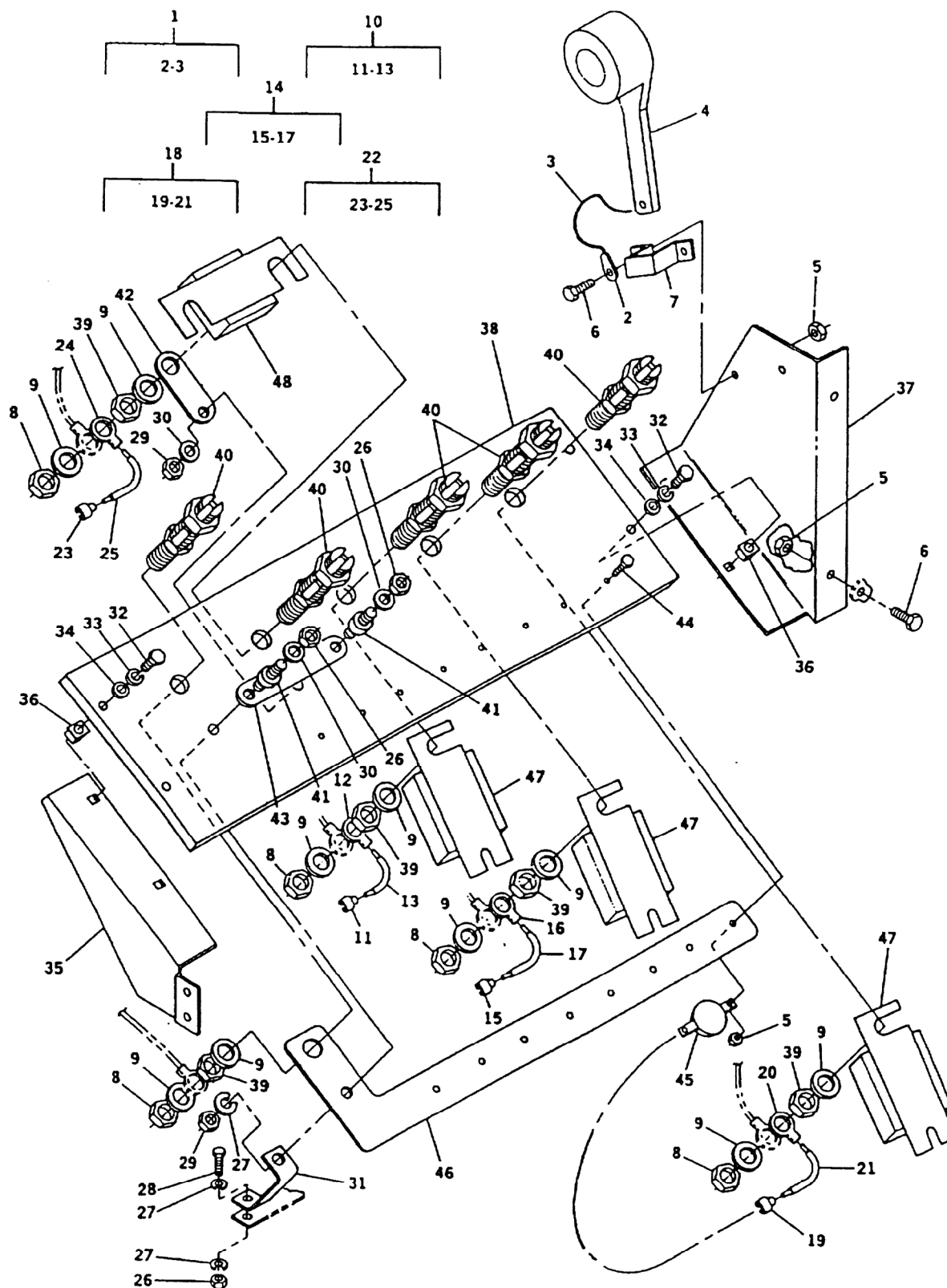
Figure 17. Load Terminal Board.
