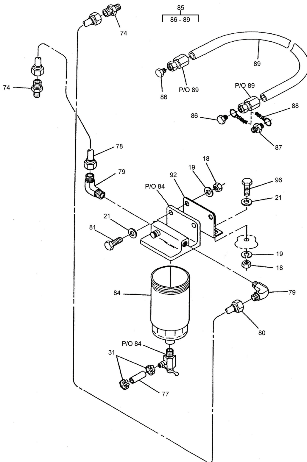
Figure 13. Fuel Tank, Lines and Fittings (Sheet 2 of 2).
