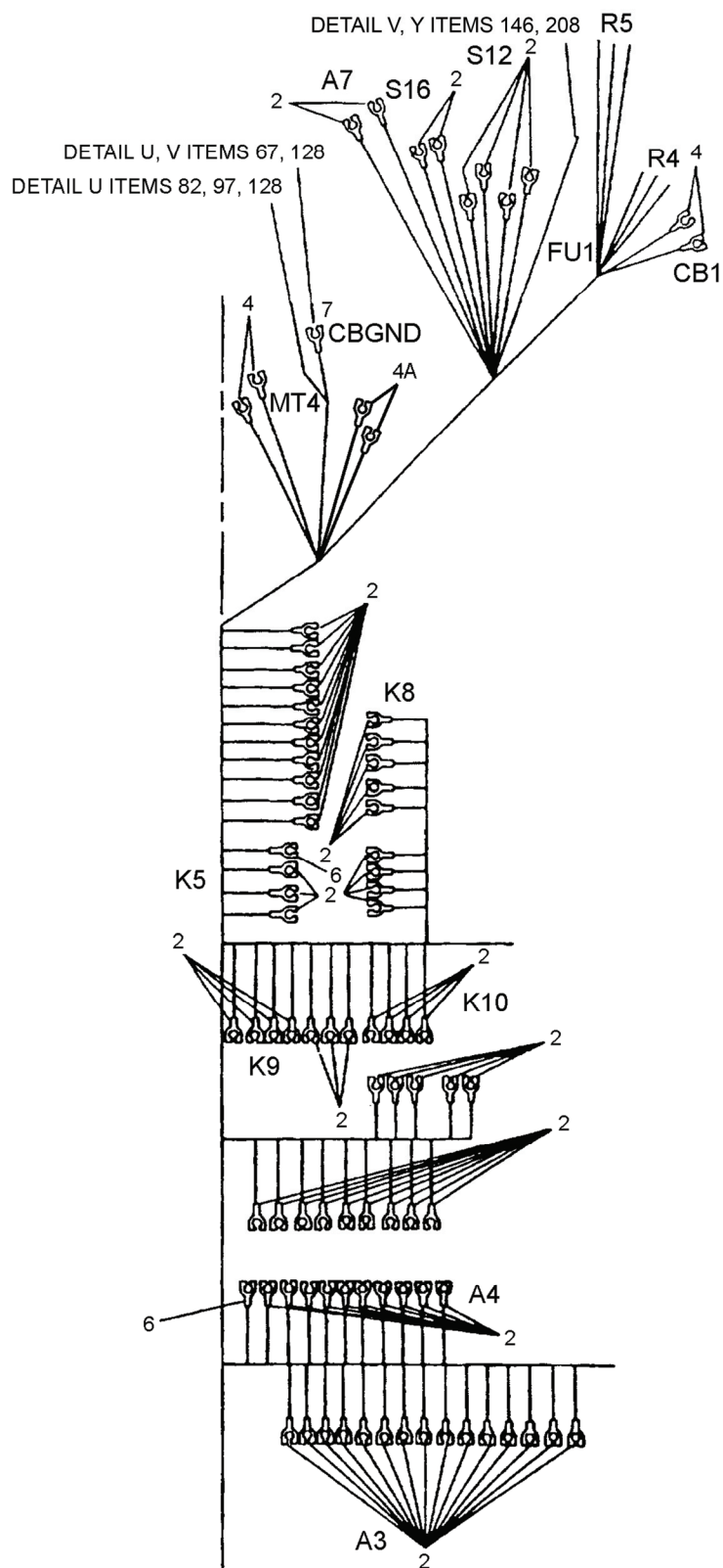
Figure 8. Control Box Harness Assembly (Sheet 3 of 25).
