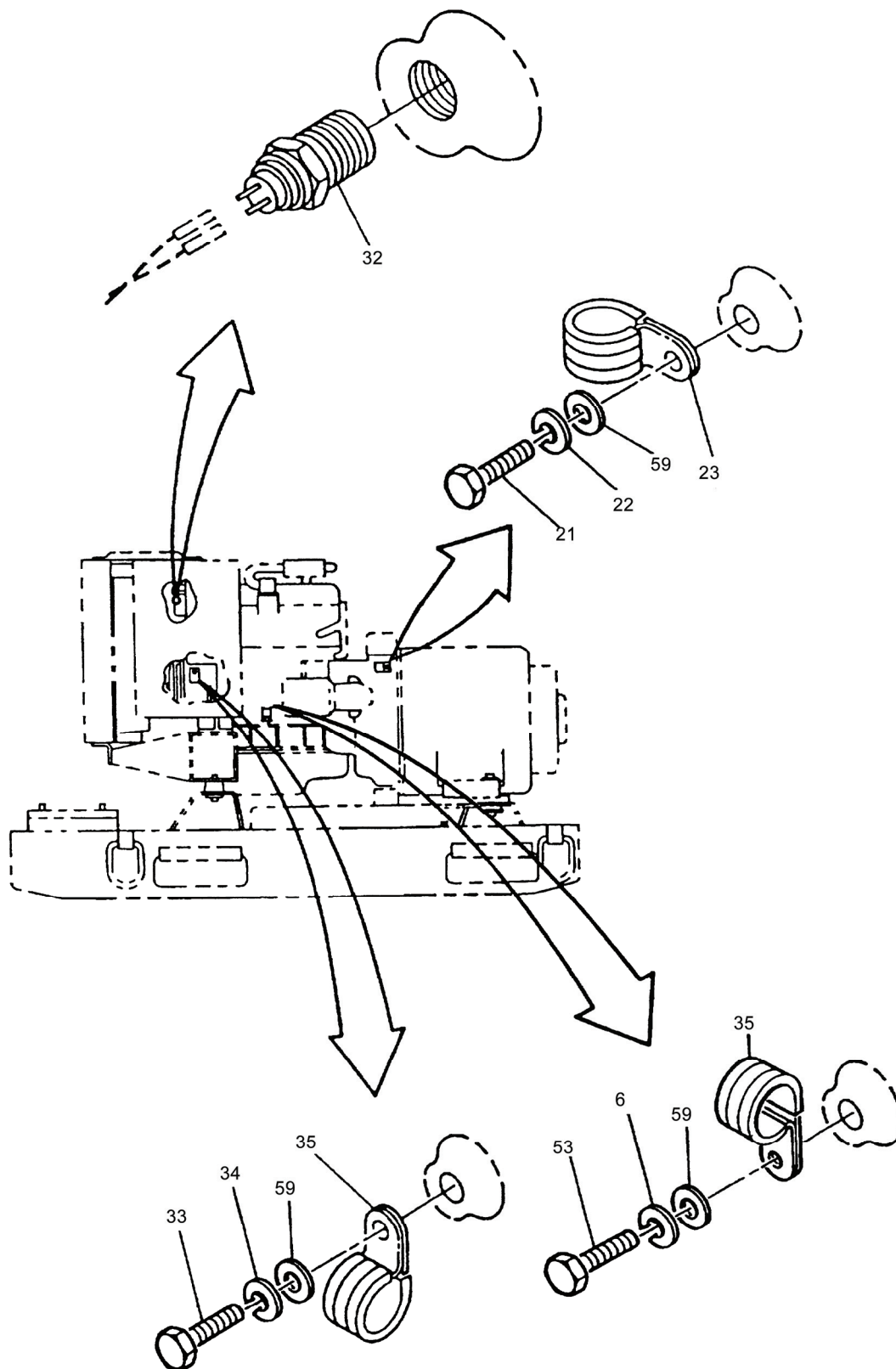
Figure 18. Engine Accessories (Sheet 3 of 5).
