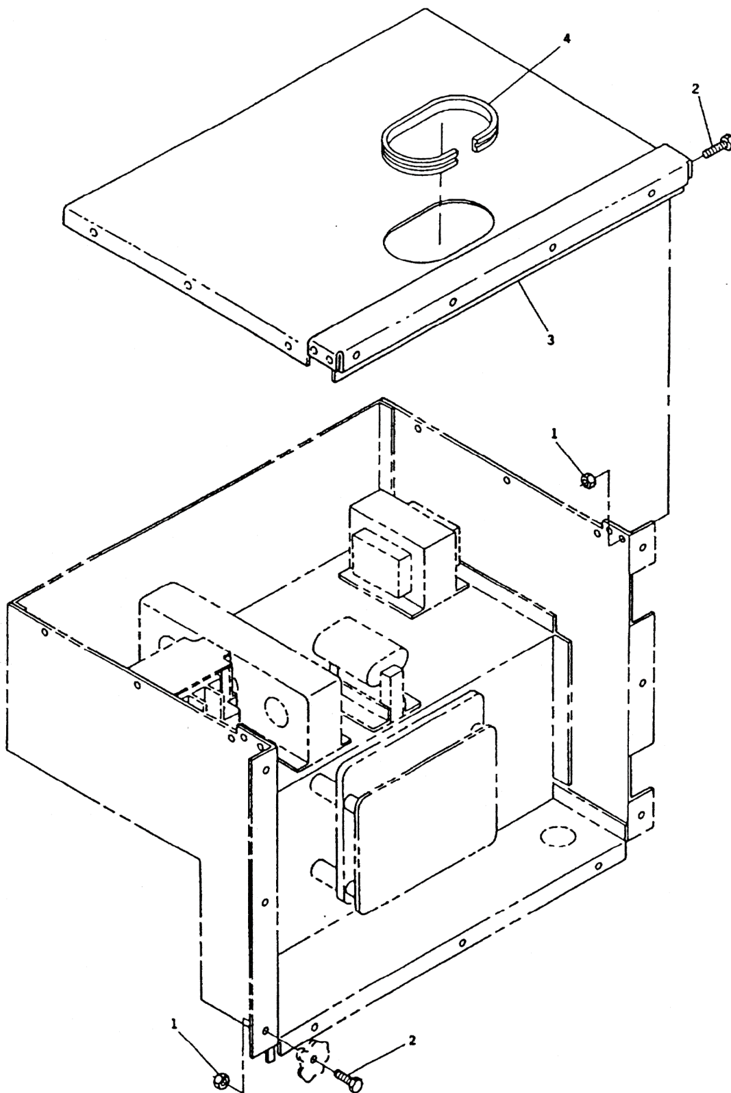
Figure 14. Output Box Installation.
