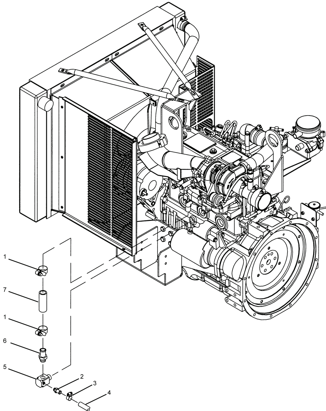
Figure 19.1. Lubrication Accessories (Sheet 1 of 2).
